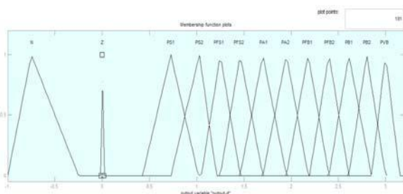
Figure 10. Linguistic variables from output signal
