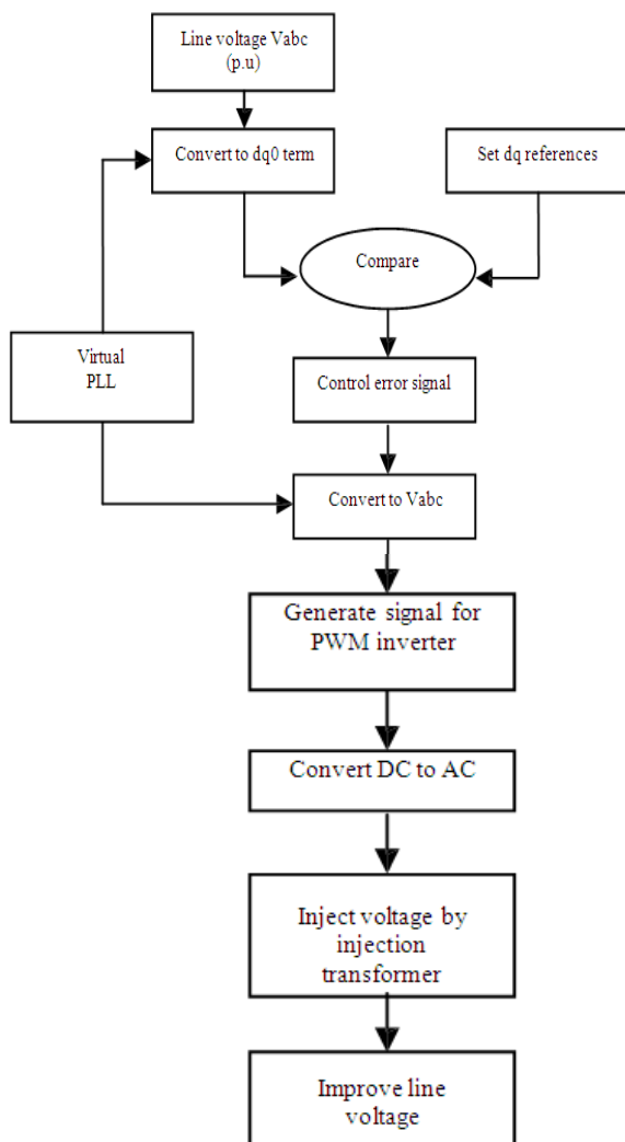
Figure 2. Flow chart of DVR operation
