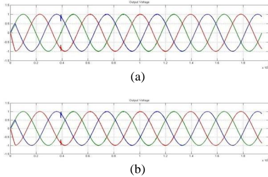
Figure 14. (a) Output voltage at load 1 after injection voltage from DVR controlled by PI; (b) Output voltage at load 1 after injection voltage controlled by FL.
