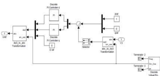
Figure 5. Control circuit using PI controller
