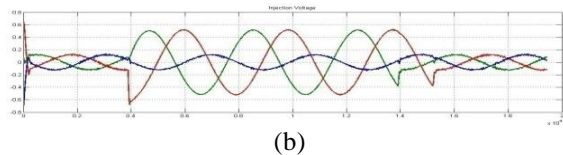
Figure 11. (a) Injection voltage from DVR controlled by PI; (b) injection voltage controlled by FL
