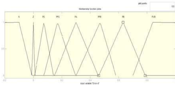
Figure 8. Linguistic variables from input
