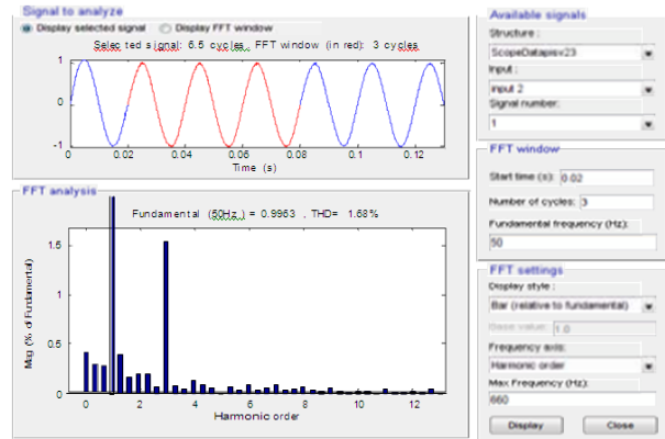
Figure 15. THD generated when PI controller is applied
