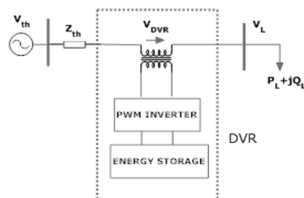
Figure 1. Calculation for DVR voltage injection
