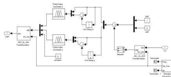
Figure 7. Control circuit using FL controller
