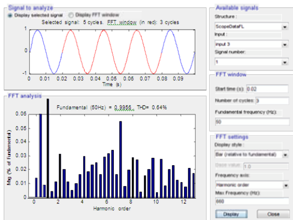
Figure 16. THD generated when FL controller is applied
