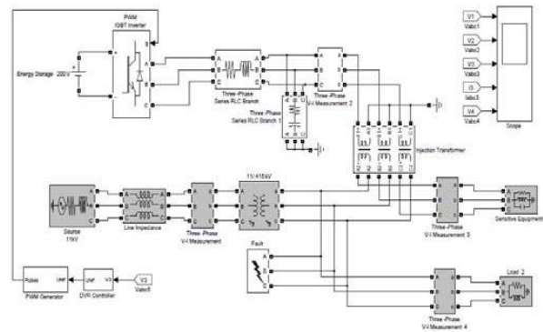
Figure34. DVR Modelling using Matlab/Simulink
