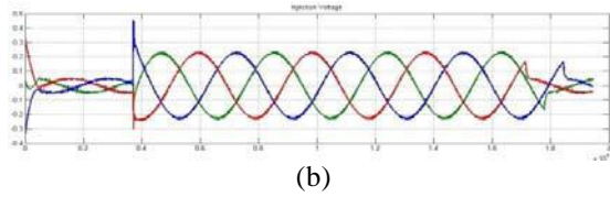
Figure 13. (a) Injection voltage from DVR controlled by PI; (b) injection voltage controlled by FL.
